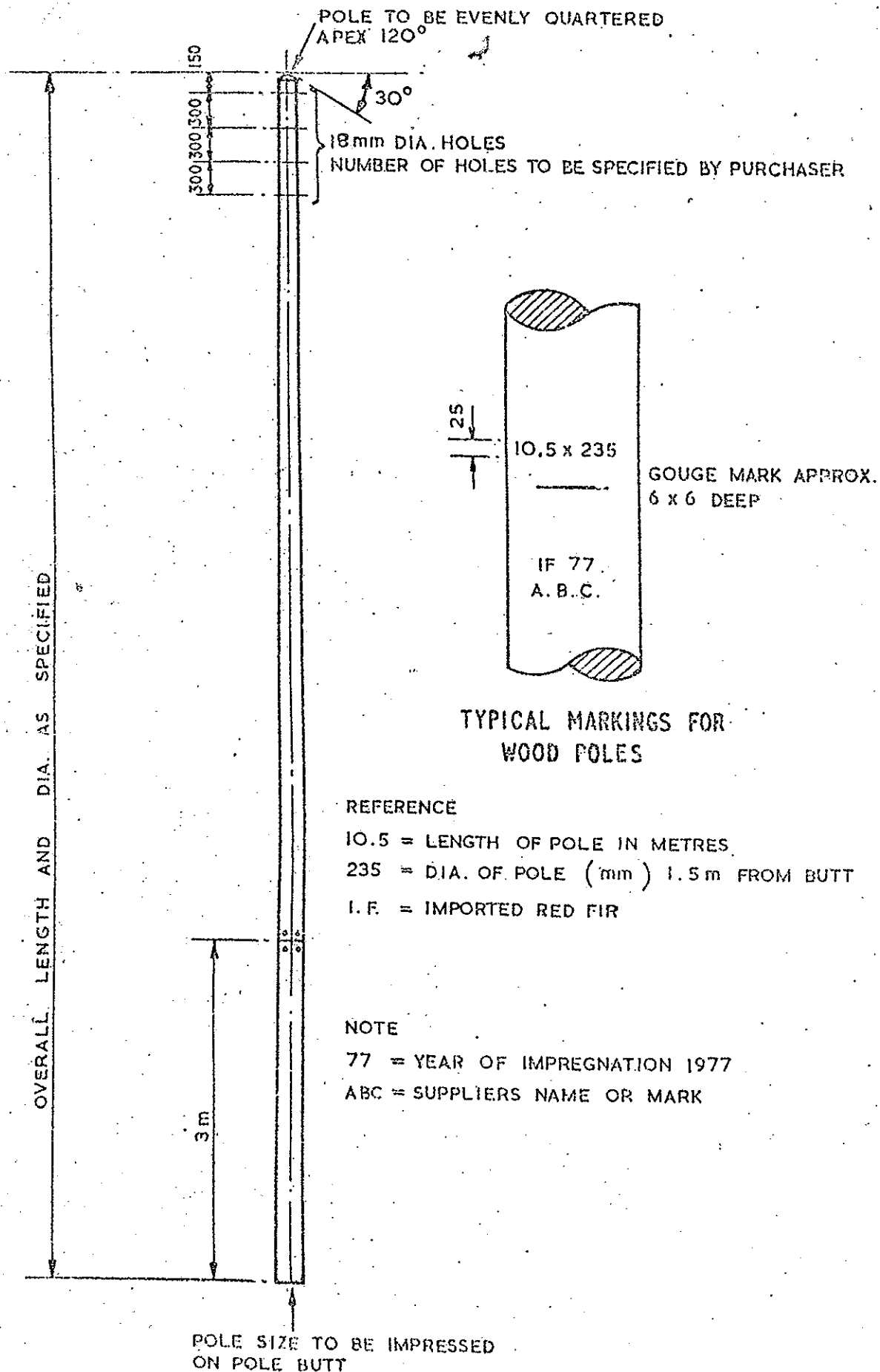
Fig. 1 Drillings and markings of wood poles for l.v. overhead lines (ESI Drawing 43300)
